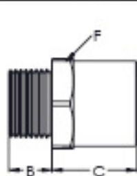
SM - Straight
