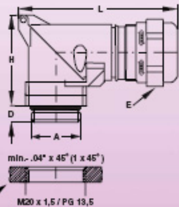
Threaded / Single Hole Connection
